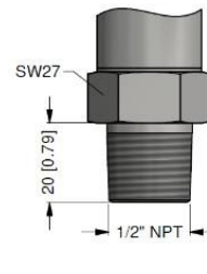
1/2" NPT
