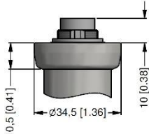
Binder Seria 723 5-pin (IP 67)
