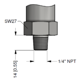
1/4" NPT
